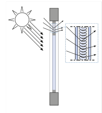
Figure 14 | Exemplary designs of light-directing sun and glare protection systems. [© Fraunhofer IBP]
