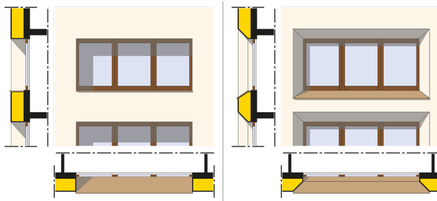
Figure 13 | Outwarded opening window reveals retain portions of previous daylighting when façade is insulated. [© Fraunhofer IBP]
