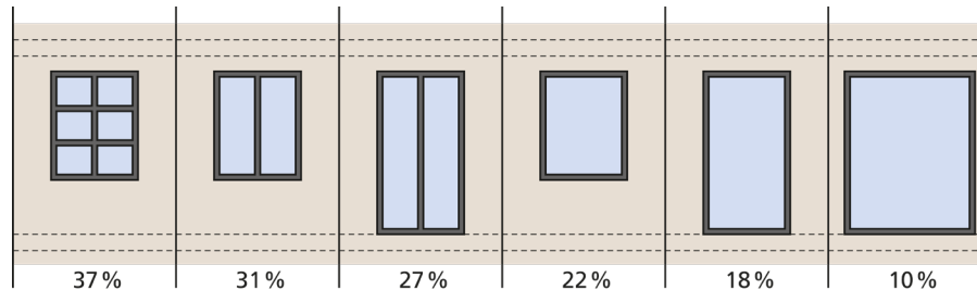
Figure 12 | Comparison of different frames with indication of the respective frame share in the clear opening. [© Fraunhofer IBP according to data from https://www.energie.ch ]
