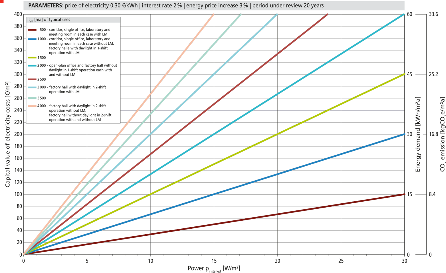
Figure A.1 | Capital value of electricity costs, energy demand and CO 2 emission as a function of installed power and operating time. [© Fraunhofer IBP]
