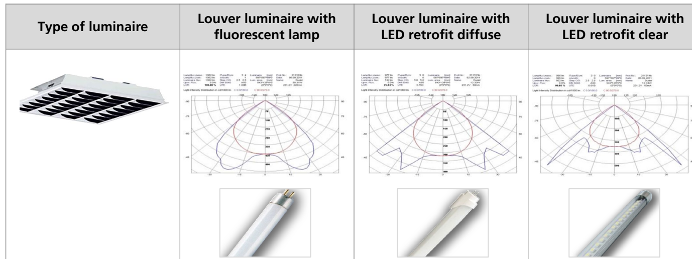
Figure 11 | Example of the changed light distribution when replacing fluorescent lamps with LED retrofit “LED tubulars” for an office room louver luminaire. [© Fraunhofer IBP, TRILUX]
